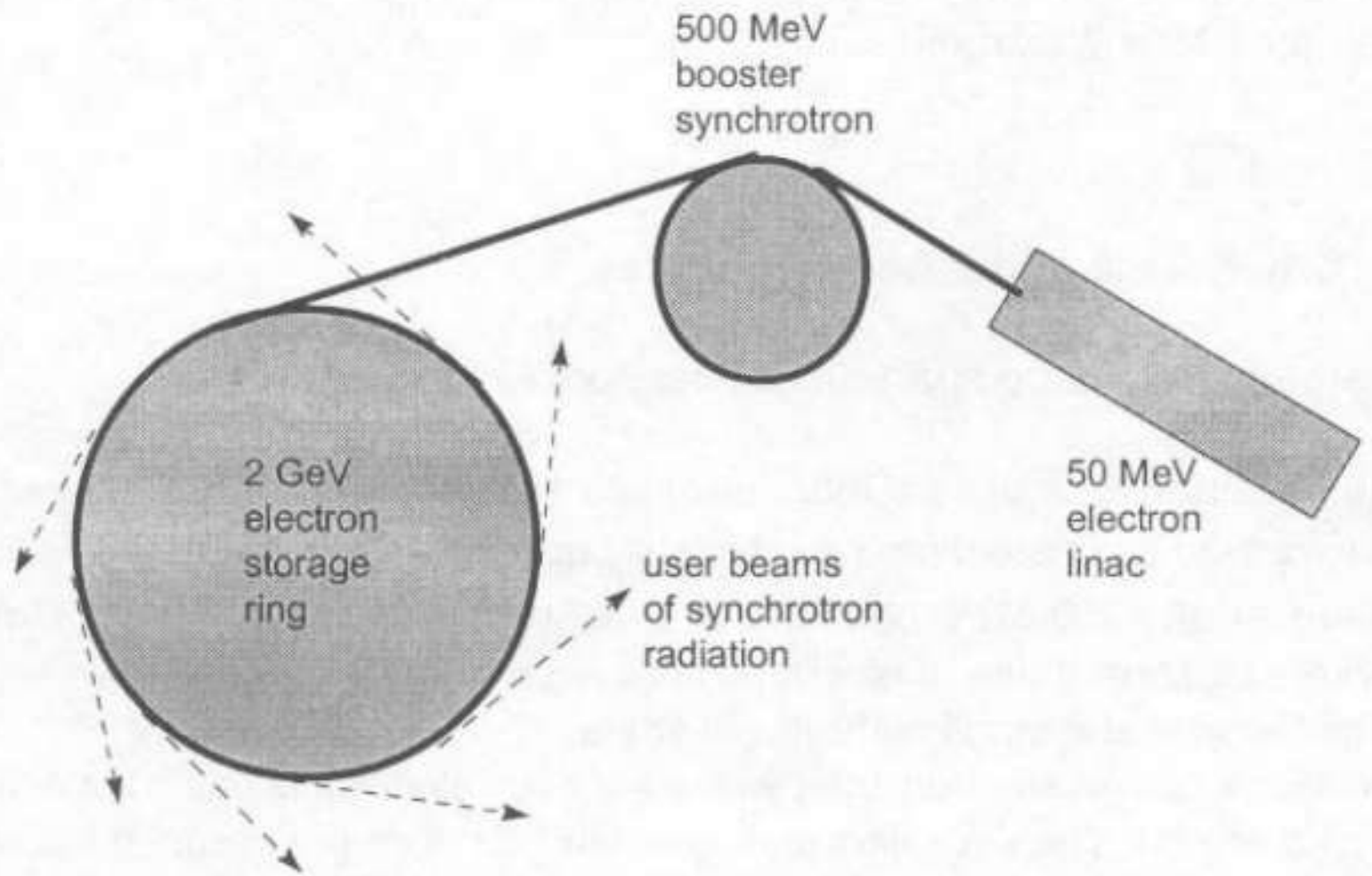
Fig. (1.27) A typical electron storage ring used to produce synchrotron radiation.
